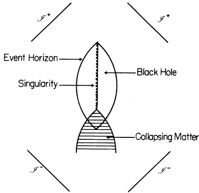
FIG. 1. A gravitational collapse produces a black hole which slowly evaporates by the emission of radiation to future null infinity \mathcal{I}^+ . Because of the loss of energy, the black hole decreases in size and eventually disappears.
