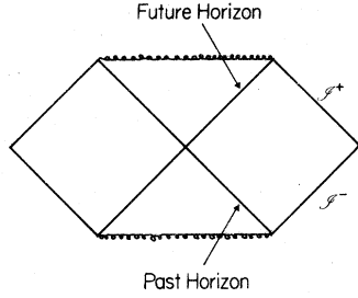
FIG. 3. The Penrose diagram of the r - t plane of the analytically extended Schwarzschild space. Null lines are at \pm 45^\circ and a conformal transformation has been made to bring infinity, represented by \mathcal{S}^+ and \mathcal{S}^- , to a finite distance. Each point in this diagram represents a sphere of area 4\pi r^2 .
